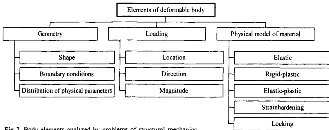
Fig 2. Body elements analysed by problems of structural mechanics
